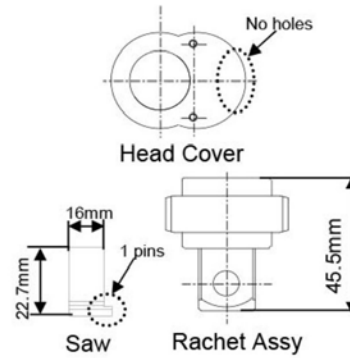
RRK-QL420Nv2.1 The head cover is included
